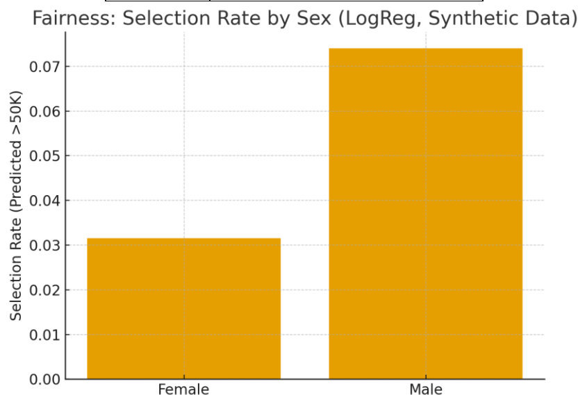
Figure 4: Selection Rate by Sex (Logistic Regression)
