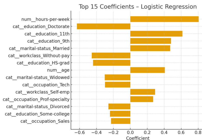
Figure 3: Top 15 Logistic Regression Coefficients
