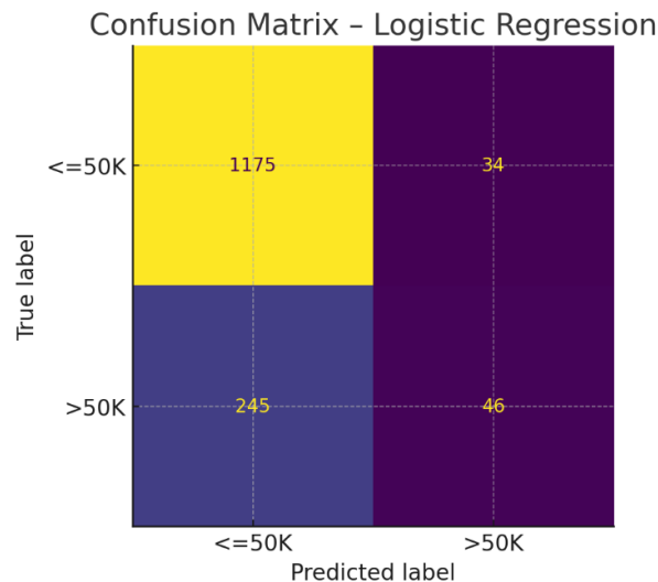
Figure 3: Confusion Matrix – Logistic Regression
